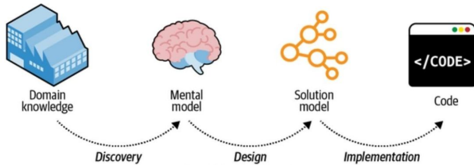
Figure 2-2. Model transformations
